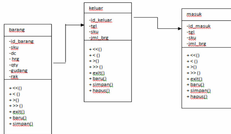
Gambar 5. Rancangan Basis Data Logikal
