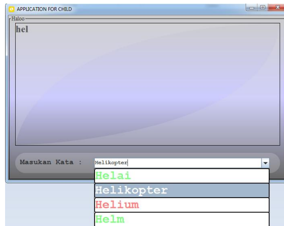
Gambar 3. Checker Kata
